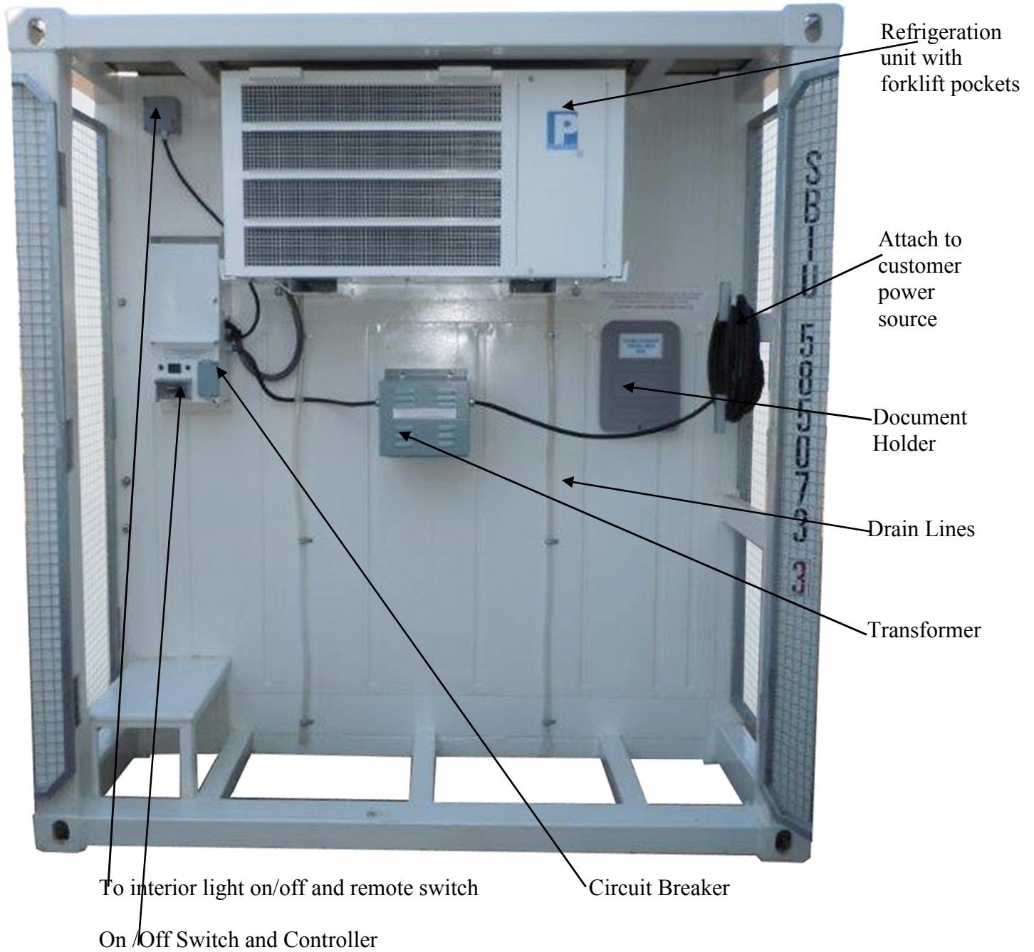
Figure 2 Component Identification
